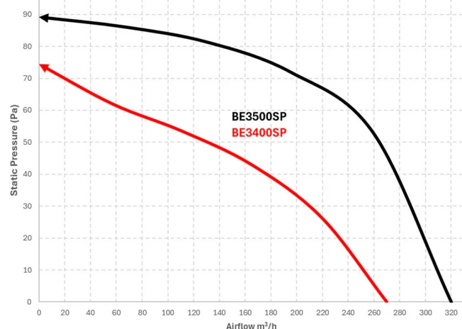
Pressure Curve for Novaline II Round
