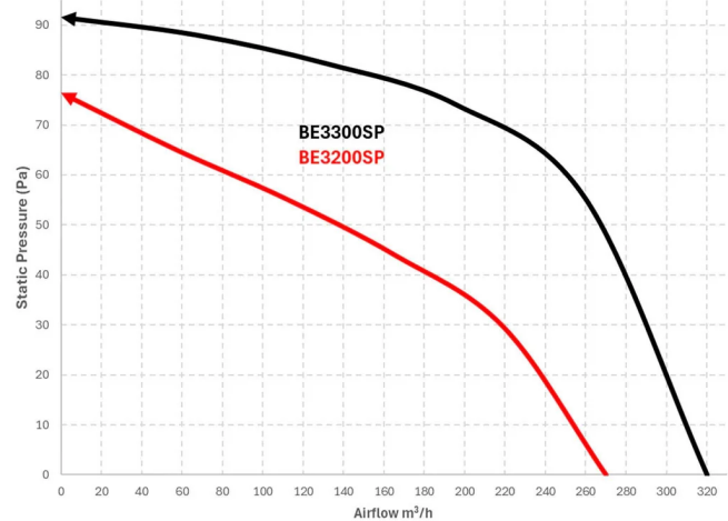
Pressure Curve for Novaline II Square
