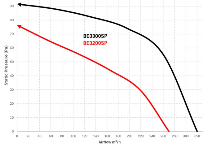
Pressure Curve for Novaline II Square
